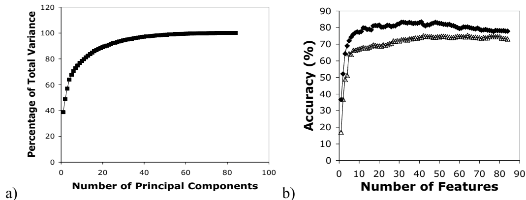
Figure 3. Feature reduction using PCA and NLPCA. (a) Variance captured by increasing numbers of sorted principal components. (b) Classification accuracy using SVM after feature reduction by PCA (◆) or NLPCA (Δ).
