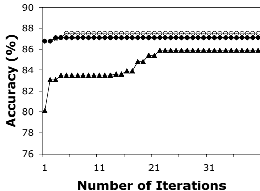
Figure 8. Feature selection using Genetic Algorithms with random feature subsets( \circ ), SLF8 subset( \blacklozenge ), and SLF10 subset( \blacktriangle ) as the starting populations.
