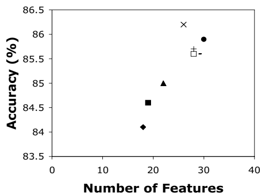
Figure 7. Feature selection using FDR with different threshold parameters: 0.1( \blacklozenge ), 0.08( \blacksquare ), 0.04( \blacktriangle ), 0.02( \times ), 0.01( \square ), 0.008(+), 0.004(-), 0.001( \bullet ).
