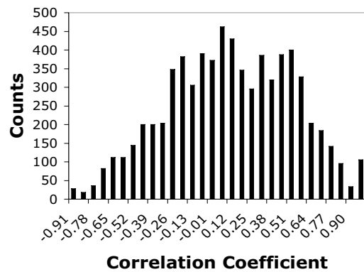
Figure 2. Histogram of all pair-wise feature correlation coefficients in SLF7.
