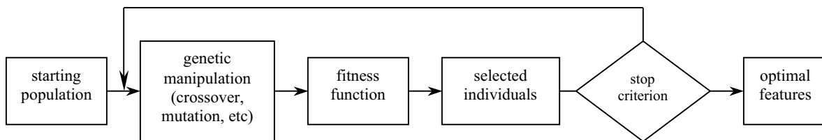
Figure 1. Flow chart of feature selection using genetic algorithm
