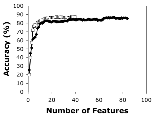
Figure 6. Feature selection using SDA ( \square ) and Classification Tree information gain ratio ( \blacklozenge ).
