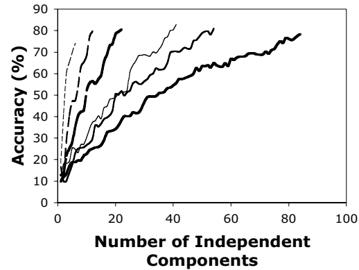
Figure 5. Feature reduction using ICA with different preprocessing levels as described by the number of principal components and the corresponding percentage of variance: 6PC-70% (thin dashed line), 12PC-80% (medium dashed line), 22PC-90% (thick dashed line), 41PC-97% (thin solid line), 54PC-99% (medium solid line), 84PC-100% (thick solid line).
