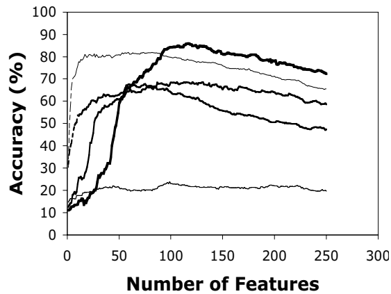
Figure 4. Feature recombination using KPCA with different kernel variances: 100 (thin dashed line), 10 (medium dashed line), 1 (thin solid line), 0.1 (medium solid line), 0.01 (thick solid line).
