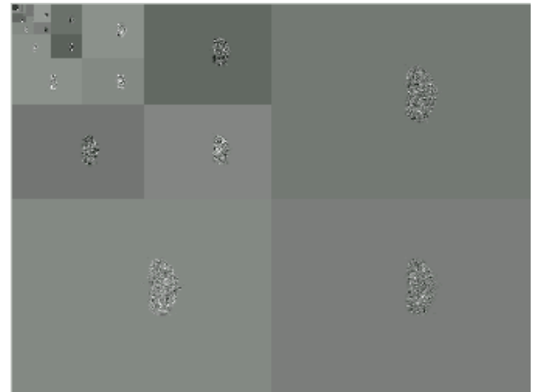
Wavelet Transformation
