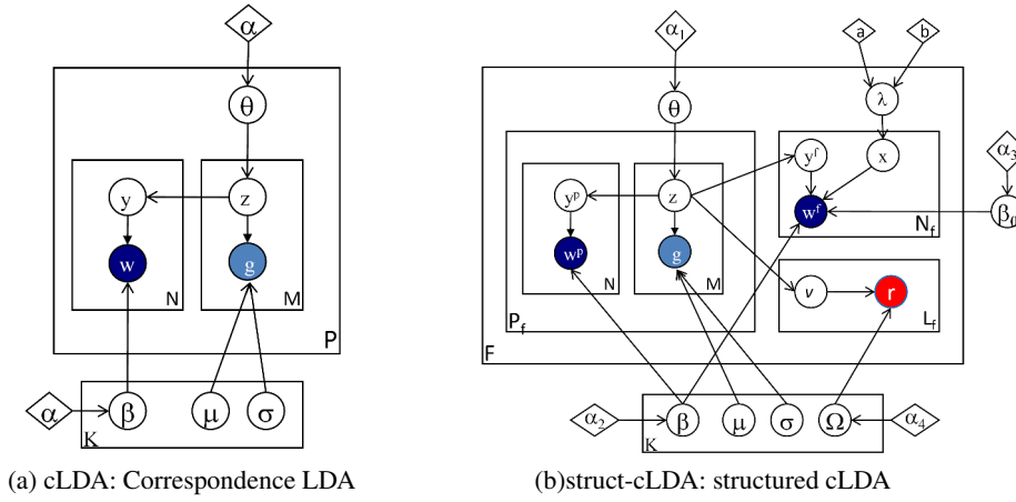
Figure 2: The cLDA and struct-cLDA Models. Shaded circles represent observed variables and their colors denote modality (blue for words, red for protein entities, and cyan for image features), unshaded circles represent hidden variables, diamonds represent model parameters, and plates represent replications. Some super/subscripts are removed for clarity — see text for explanation.
