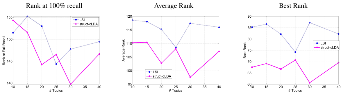
Figure 6: Evaluating protein annotation quality based on observing text and image features (Lower better)
