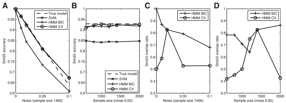
FIG. 3. (A) Testing error of simulated dataset generated from a structure with 25 states with varying levels of noise (false positive and false negative in features). The training sample size was fixed at 1400. (B) Testing error versus different training sample sizes. The noise level was fixed at 2%. (C) The ratio of overlapping nodes and edges between the learned model and the true model with varying levels of noise. The training sample size was fixed at 1400. (D) The ratio of overlapping nodes and edges with varying training sample sizes. The noise level was fixed at 2%.
